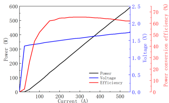
Power-Current-Voltage-Efficiency
