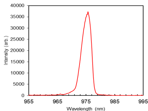
Spectral characteristics
